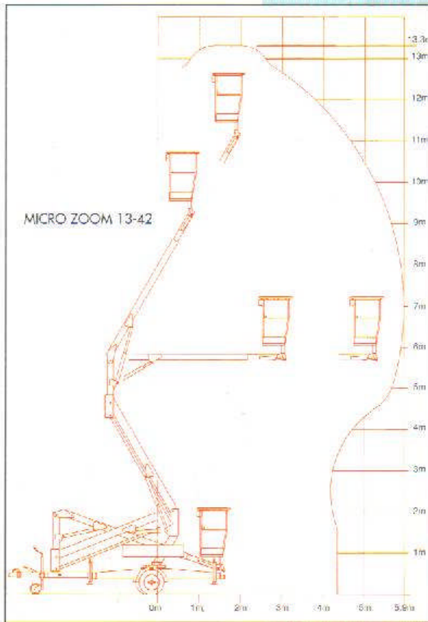
Working Envelope for MZ 13-42
